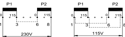
Primary connections
