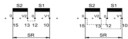
Secondary connections
