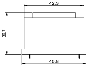
SINGLE SECONDARY, 8VA. Ta70B
