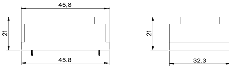
SINGLE SECONDARY, 2,4VA. Ta°70B
